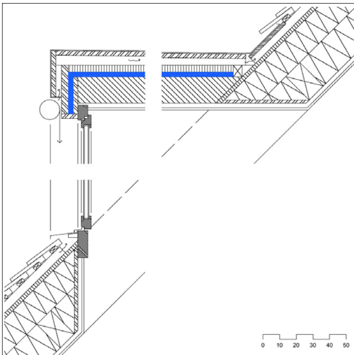
Figure 3: Section through a prefabricated dormer window for the renovation of an old building (Architect: Viridén + Partner, Zurich, Switzerland)
