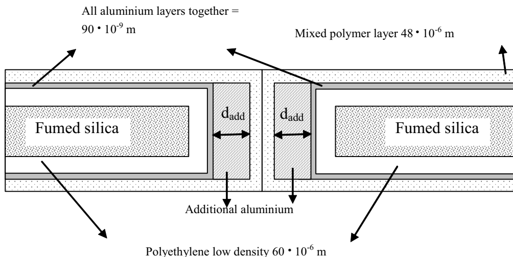
Figure 11: Section through a VIP. Simplified model of the VIP for numerical calculations
