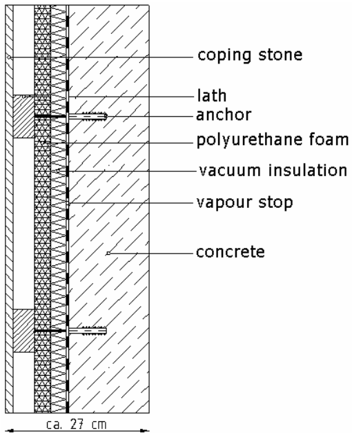
Figure 61: Left: Intended design for the prefabricated wall elements. An average U-value of 0.15 \text{ W}/(\text{m}^2\cdot\text{K}) is achieved with a total thickness of only 27 cm. Right: Photo of a prefabricated wall element
