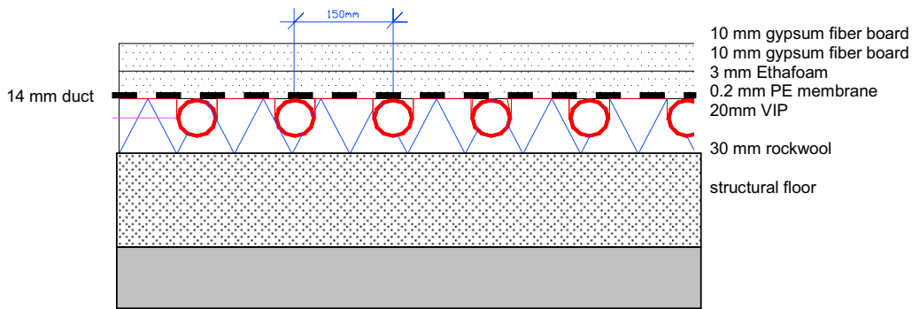
Figure 88: Principle construction layout of an acoustically improved dry VIP based floor heating system (concept 1)
