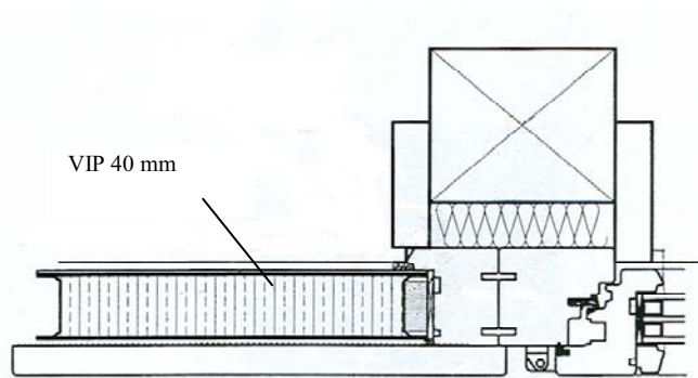
Figure 38: Left: Horizontal section through the construction Right: Installation of the VIP
