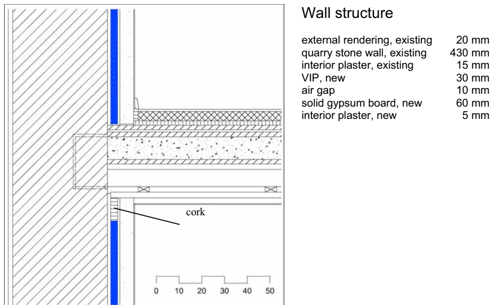
Figure 71: Section through the support of the ceiling
