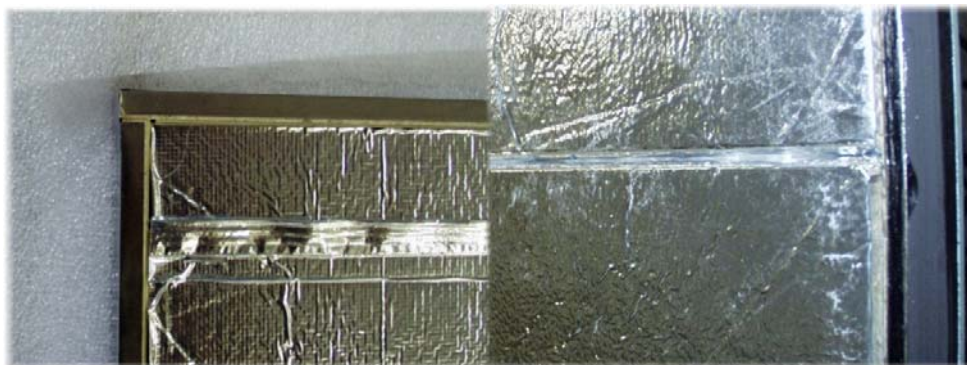
Figure 57: Gaps and edges of VIP in the elements left: va-Q-tec AG VIP right: WACKER CHEMIE VIP
