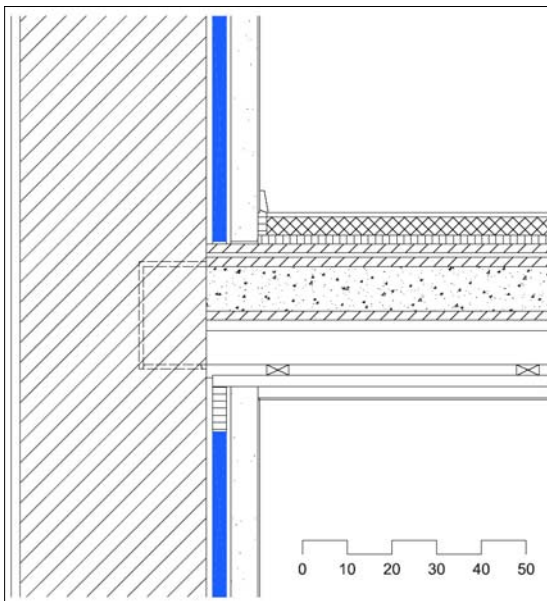
Figure 24: Vertical section through the Brick outer wall with interior insulation
