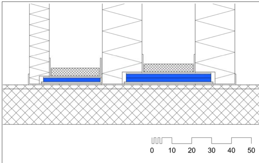
Figure 31: Vertical section of a cold (left) and a deep-freeze room (right)
