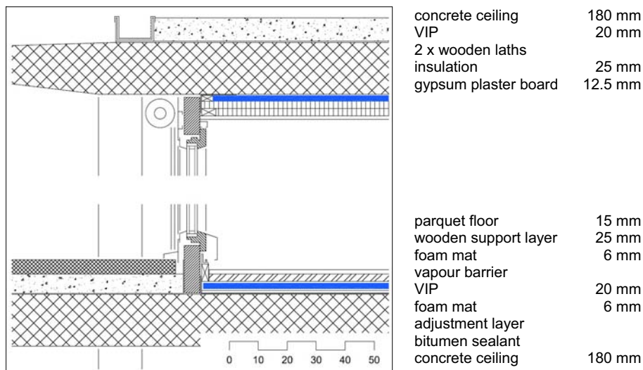
Figure 20: Vertical section, joint between the VIP construction and the window front
