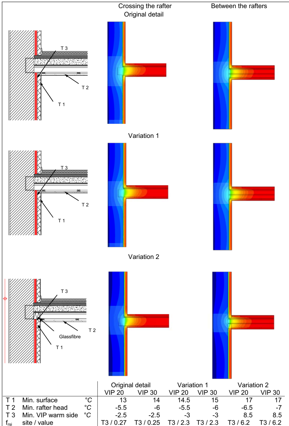
Figure 72: Three-dimensional computational heatflow analysis of the support of the ceiling
