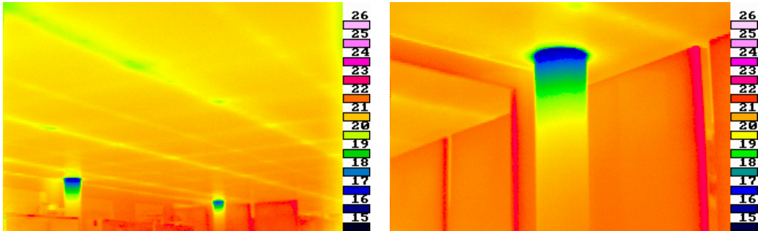
Figure 21: Concrete pillars passing from the roomside through the VIP-layer to the outside concrete roof slab. Pictures with the IR-Camera
