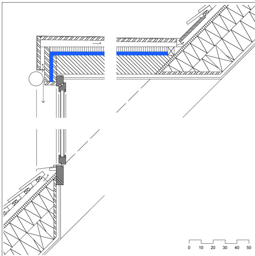
Figure 80: Vertical section through a prefabricated dormer window for the renovation of an old building
