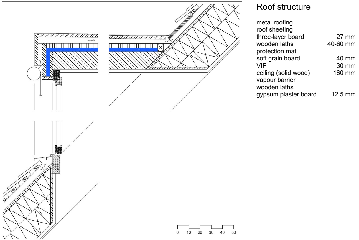
Figure 26: Section through the dormer window construction
