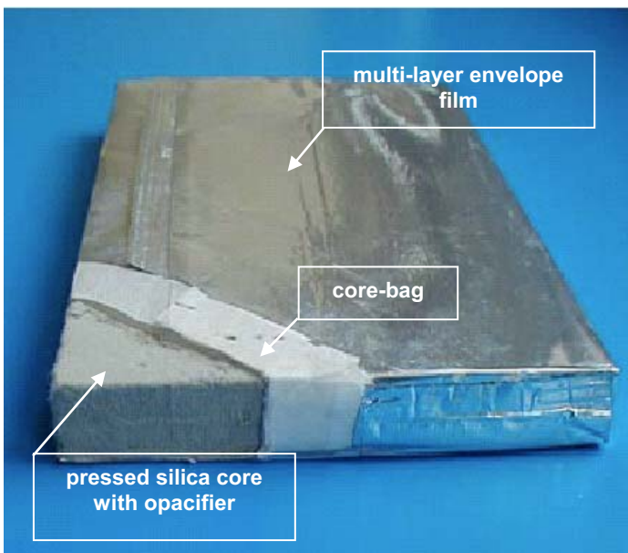
Figure 6: Components of a VIP. The core-bag provides mechanical stability for handling and protects the welding area from being polluted by core-powder. (foto: va-Q-tec)
