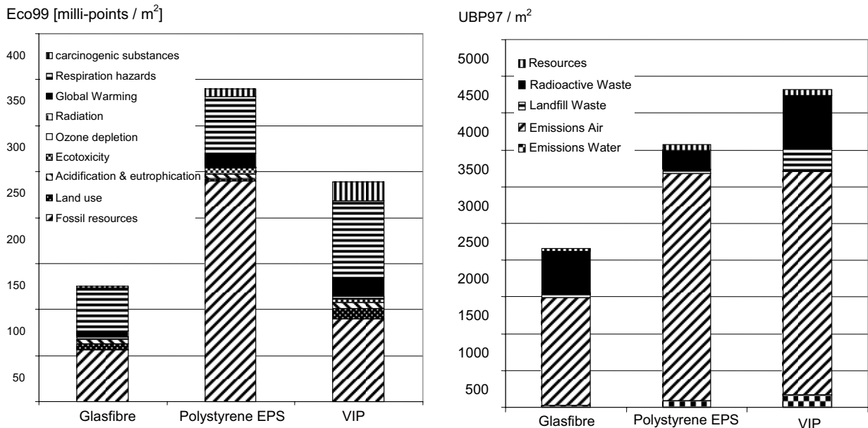
Figure 18: Left: Comparison of the categories of effects for the insulating materials glass wool, polystyrene EPS and VIP according to the method Eco-indicator 99 Right: Comparison of the insulating materials glass wool, polystyrene EPS and VIP according to the Method of Ecological Scarcity with environmental pollution points UPB 97
