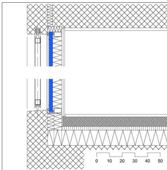
Figure 33: Section of façade with VIP-Multiplac wall elements
