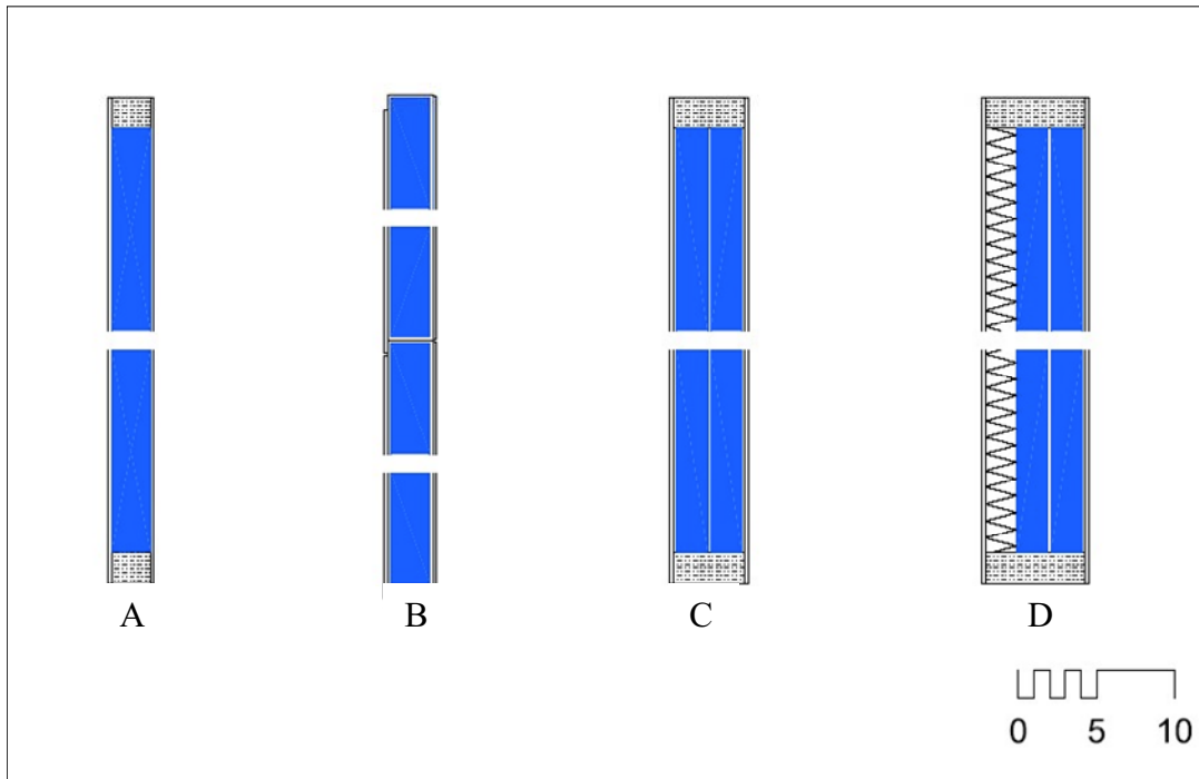
Figure 35: VIP-MULTIPLAC elements
