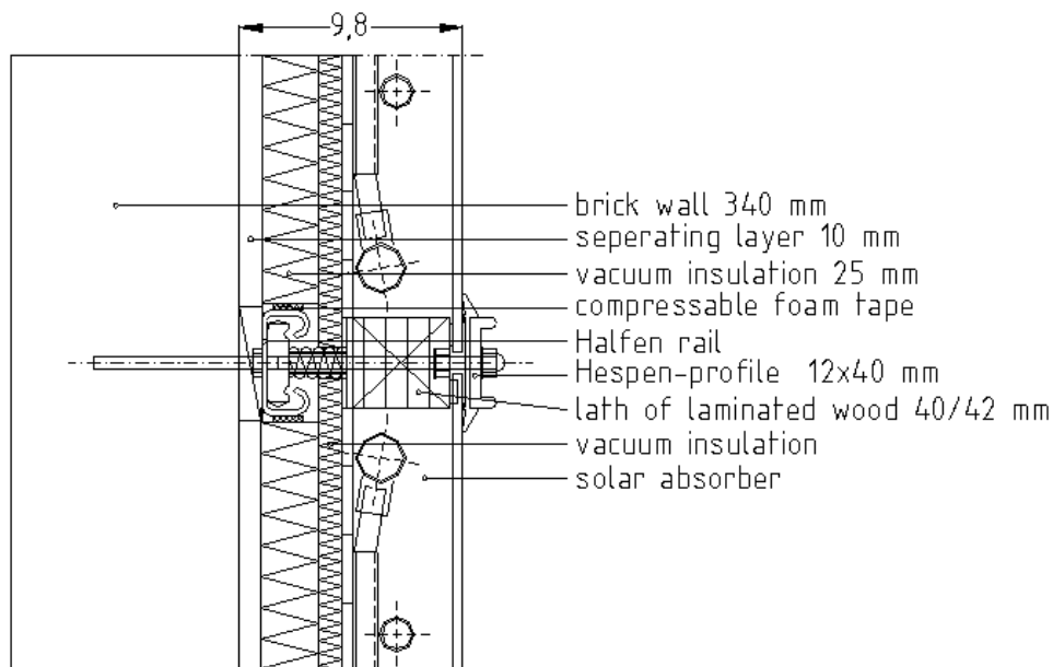
Figure 49: Cross-section of the south wall
