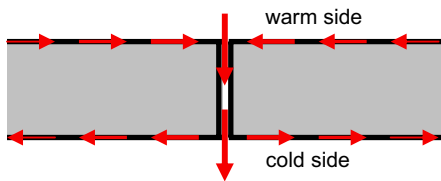
Figure 7: Schematic representation of a cold bridge between two VIP
