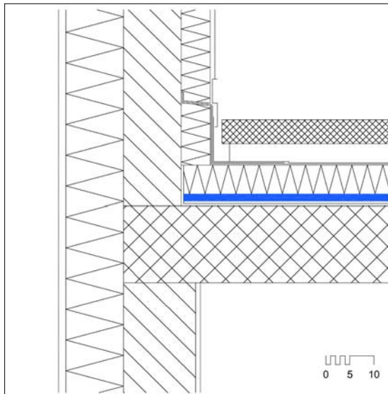
Figure 28: Vertical section through the joint detail at parapet
