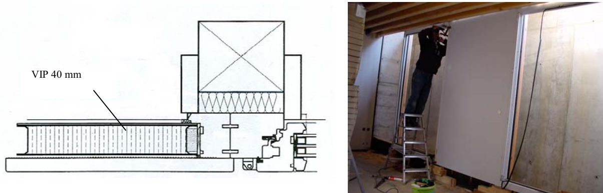
Figure 4: Vacuum insulation panels in the form of stainless steel cases used as outside wall elements on single-family terrace houses in Binningen / Switzerland
