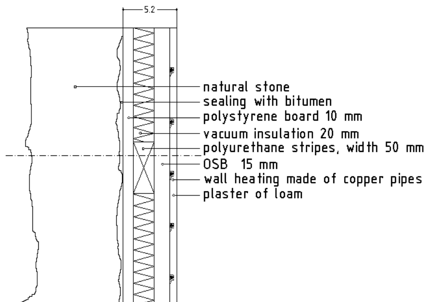
Figure 51: Cross-section of the wall
