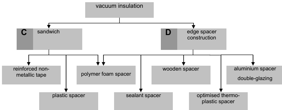
Figure 15: Overview of different edge spacers
