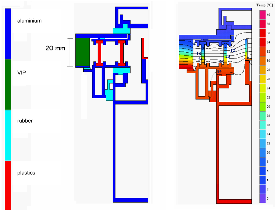
Figure 59: Left: Cross-section of the façade element without the radiator. The jamb-crossbar construction can be seen on the right hand side. The VIP is cut off on the left side. Right: A Finite-Element-Program was used to simulate the temperatures shown in this cross-section. The temperatures are colour-coded and the isotherms drawn in.
