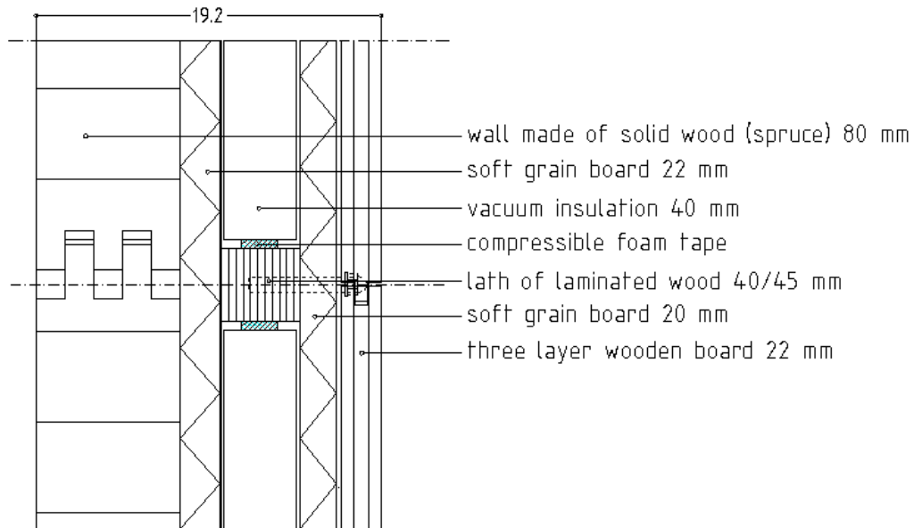
Figure 44: Cross-section of the northern wall
