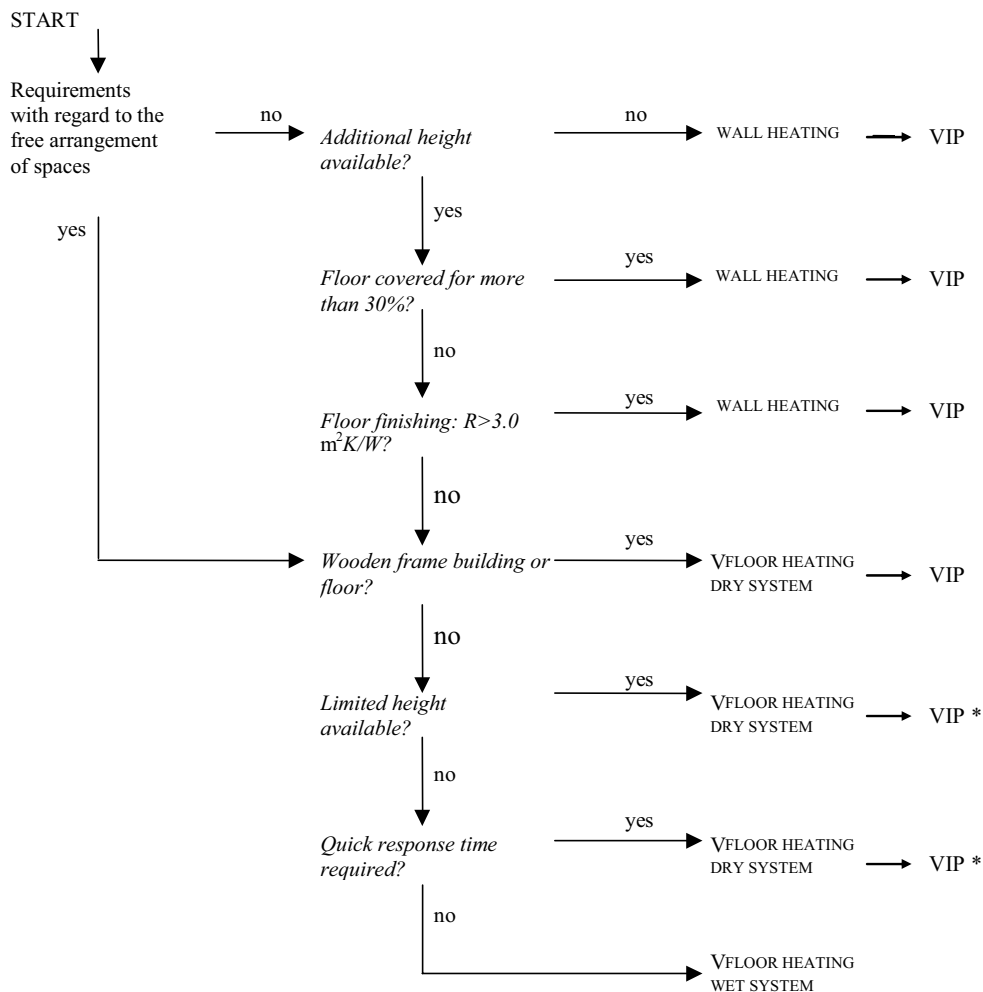
Figure 85: Decision model for low temperature heating systems
