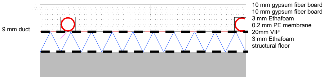
Figure 87: Principle construction layout of dry VIP based floor heating system (concept 2)
