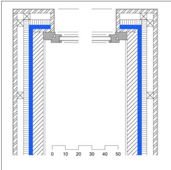
Figure 81: Horizontal section through a prefabricated dormer window for the renovation of an old building (Architect: Viridén + Partner, Zurich, Switzerland)
