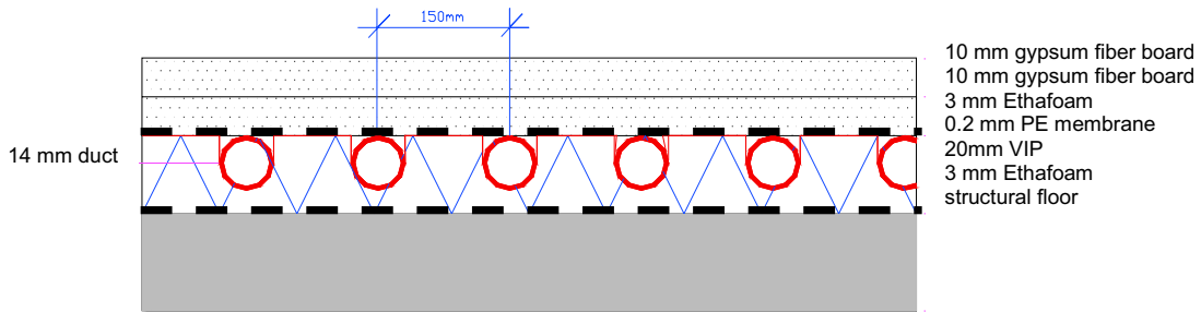
Figure 86: Principle construction layout of dry VIP based floor heating system (concept 1)
