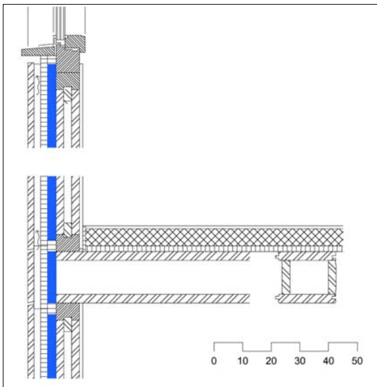
Figure 77: Vertical section through the window and the support of the ceiling
