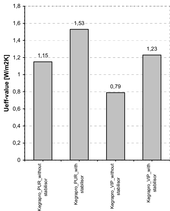
Figure 84: Effective U-value of Kegapro doors with different core materials and stabilisers
