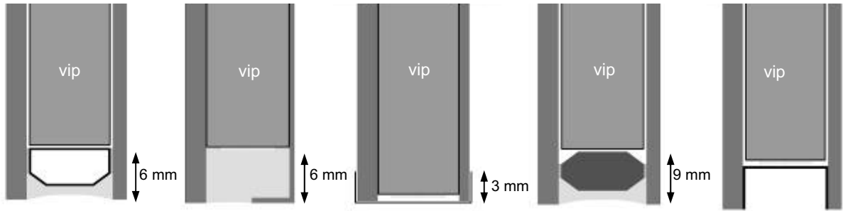
Figure 16: Different edge spacers. a.) aluminium spacer double-glazing; b.) sealant spacer; c.) reinforced non-metallic tape (0.15 mm); d.) optimised thermoplastic spacer (Henkel Tereson Thermoplastic Spacer); e.) polymer U-section
