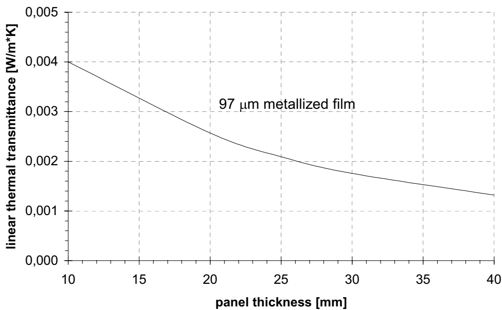
Figure 10: The effects of panel thickness on the linear thermal transmittance due to thermal bridging for a three layer metallized film; \lambda_{cop} = 4 \cdot 10^{-3} W/(m \cdot K) ), based on numerical calculation
