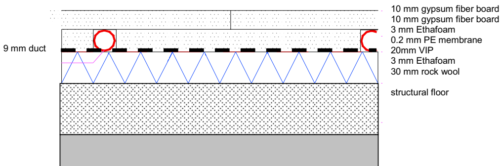
Figure 89: Principle construction layout of an acoustically improved dry VIP based floor heating system (concept 2)
