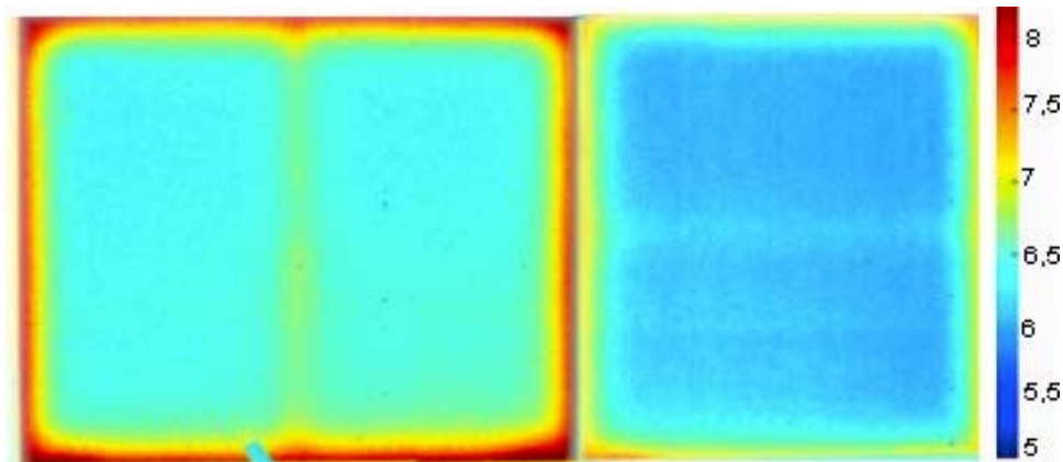
Figure 55: Infra-red image of two elements. On the left hand side the spacer is made of stainless steel and on the right hand side the spacer is made of Purenit.
