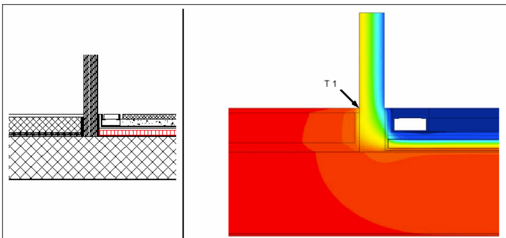
Figure 74: Vertical section through the terrace construction and three-dimensional computational heatflow analysis. The calculated temperature T1 is 14 °C.
