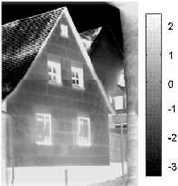
Figure 42: Infra-red image (from 2003) of the gable façade three years after the external thermal insulation composite system was installed. The edges of the VIP can be seen as lines (thermal bridges).
