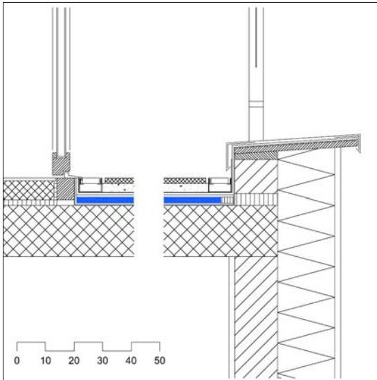
Figure 73: Section through the terrace construction
