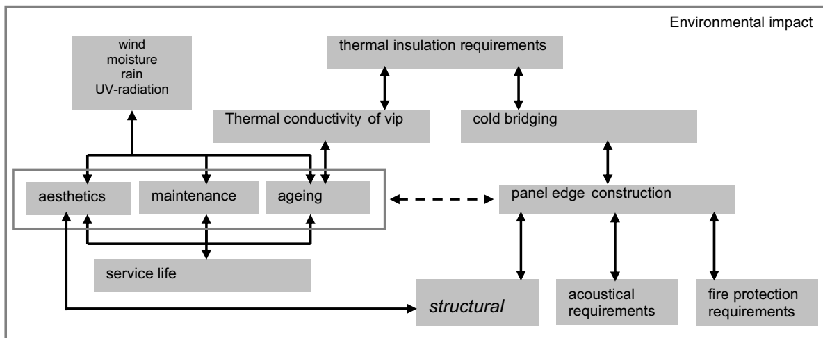
Figure 75: Relationships between different requirements for building panels with incorporated vacuum insulation panel.
