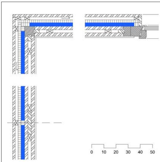
Figure 78: Horizontal section through a joint of elements, edge and window
