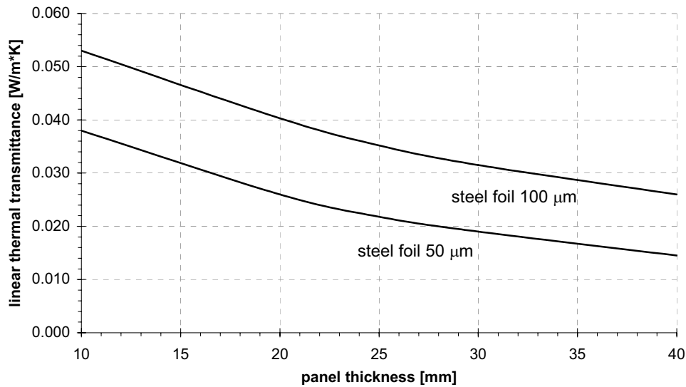
Figure 9: The effects of panel thickness and foil thickness on the linear thermal transmittance due to thermal bridging for a stainless steel foil ( \lambda_{foi} = 25 W/(m \cdot K) ; \lambda_{cop} = 4 \cdot 10^{-3} W/(m \cdot K) ), based on numerical calculation
