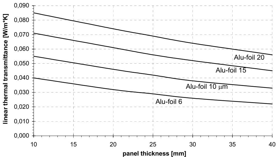
Figure 8: The effects of panel thickness and foil thickness on the linear thermal transmittance due to thermal bridging for an aluminium foil ( \lambda_{foil} = 200 \text{ W/(m·K)} ); \lambda_{cop} = 4 \cdot 10^{-3} \text{ W/(m·K)} , based on numerical calculation
