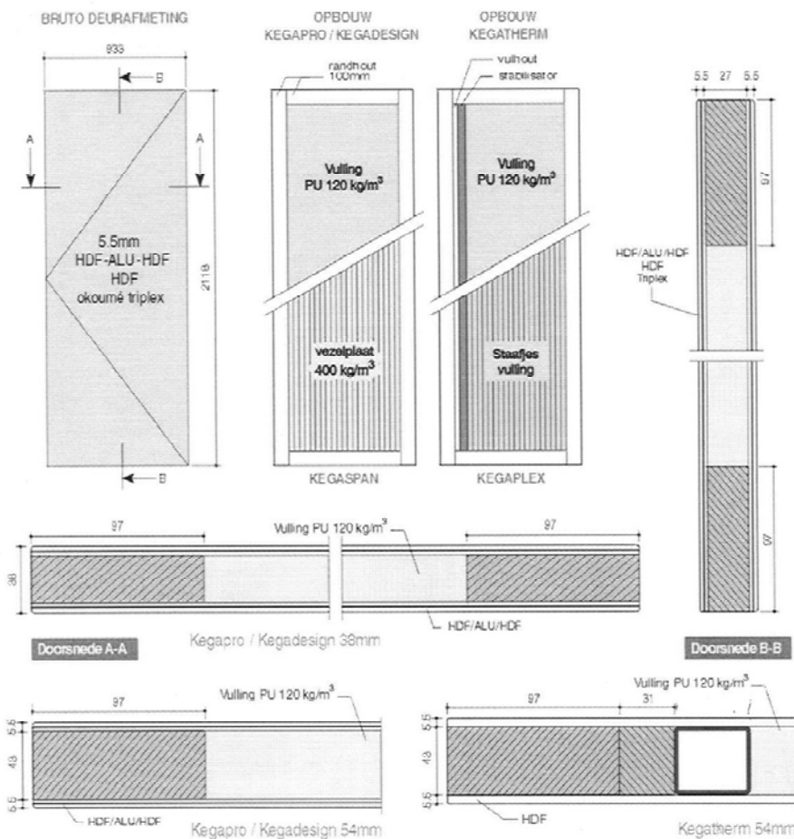
Figure 83: Overview of different door panel construction with polyurethane developed by Kegro BV in the Netherlands, source: Kegro BV
