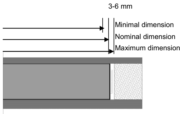
Figure 76: Tolerances in VIP integrated building components
