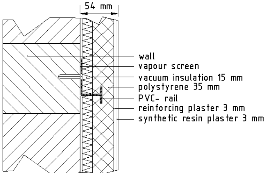
Figure 40: Cross-section of the insulated wall
