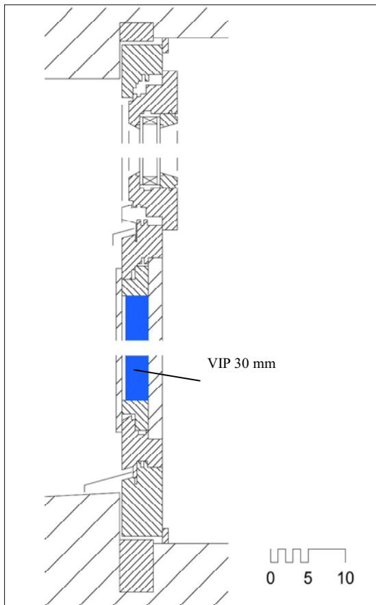
Figure 37: Parapet with VIP
