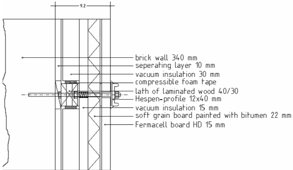
Figure 48: Cross-section of the northern wall
